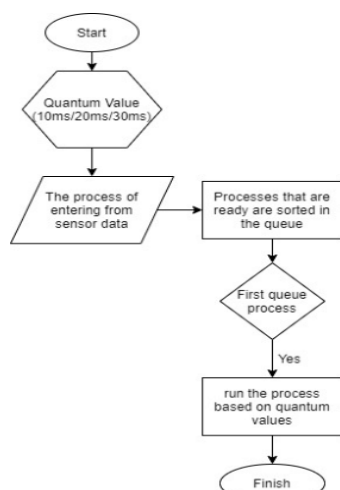
Fig. 6. Round Robin Allocation Policy
