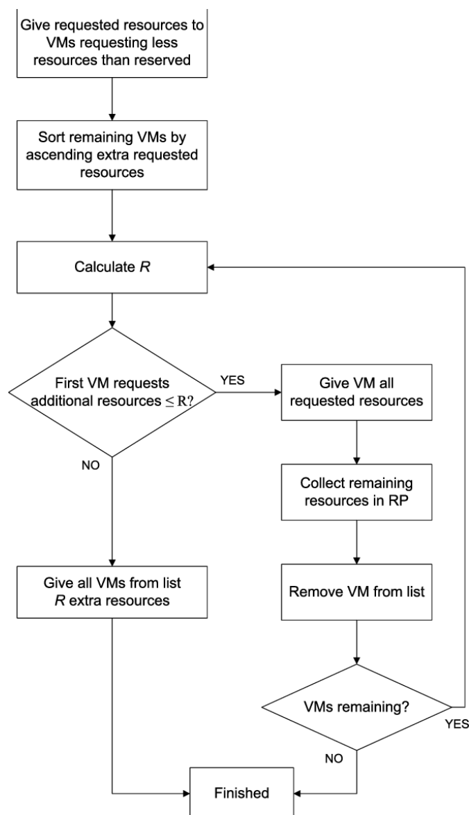
Fig. 3. Reserved Allocation Policy
