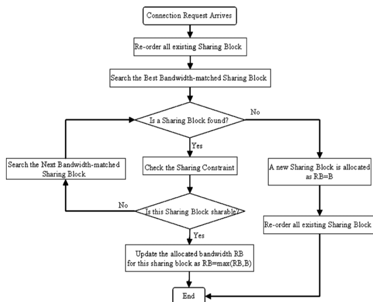
Fig. 4. Best Fit VM Allocation Policy
