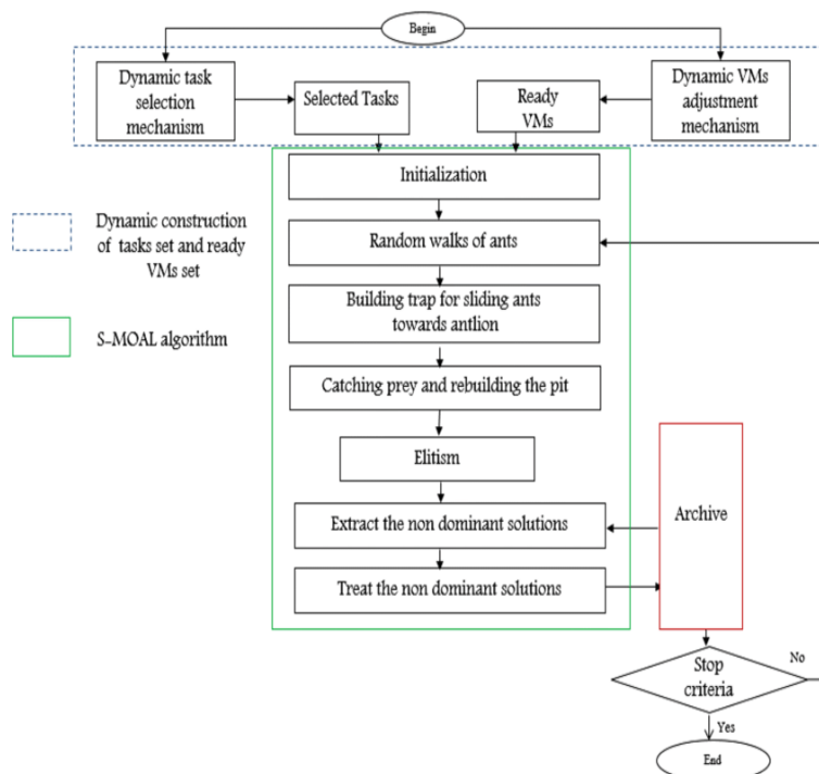
Fig. 1. Dynamic allocation policy
