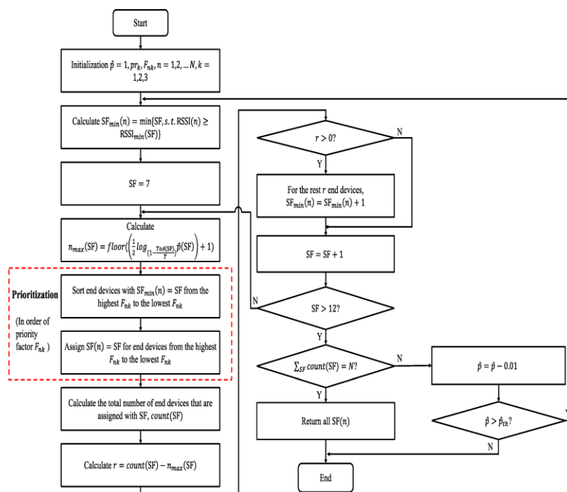
Fig. 2. Priority-Based Allocation Policy
