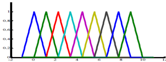
Fig (1), First degree B-spline basis function with uniform Knot vector X = \{-1, 0, 1, 2, 3, 4, 5, 6, 7, 8, 9, 10, 11, 12\}
