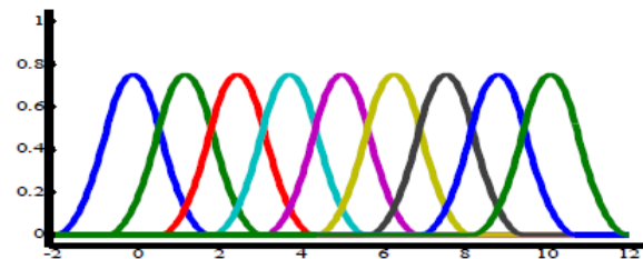
Fig (2), Second degree B-spline basis function with uniform Knot vector X = \{-2, -1, 0, 1, 2, 3, 4, 5, 6, 7, 8, 9, 10, 11, 12\}
