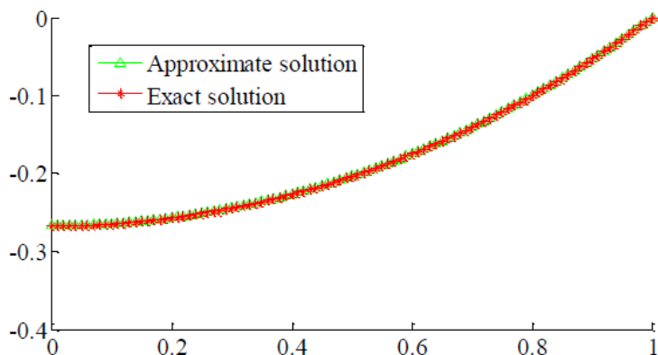
Fig (6). Comparison of approximate and Exact solutions for the Example2 for mesh size h=0.01
