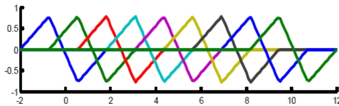
Fig (3), First derivative of second degree B-spline basis function with uniform Knot vector X= \{-2,-1, 0, 1, 2, 3, 4, 5, 6, 7, 8, 9, 10, 11, 12\}
