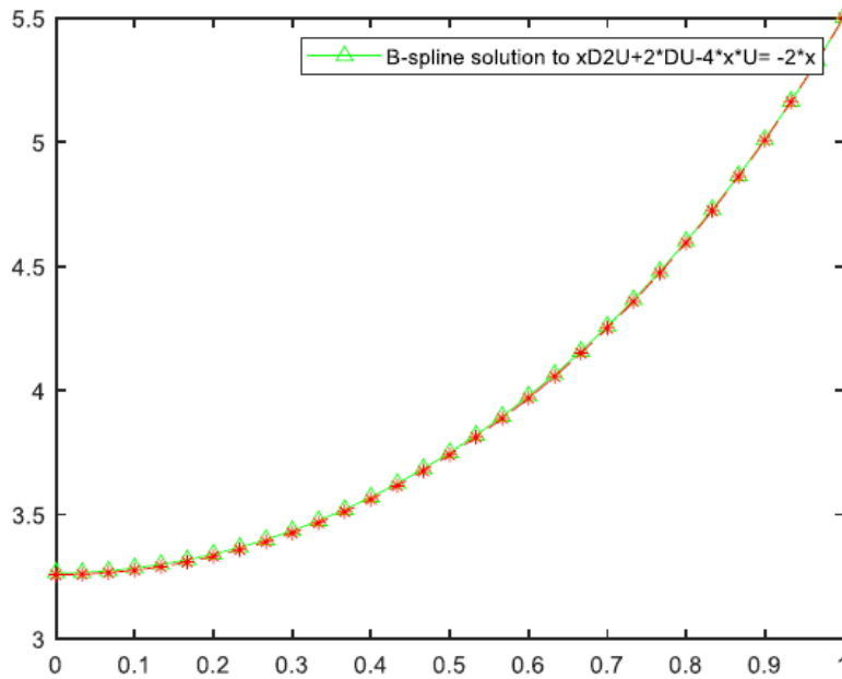
Fig(5), Comparison of the B-spline collocation and Exact solutions
