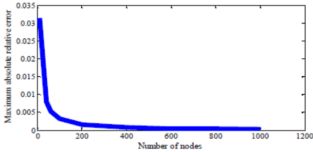
Fig (5), Trend of maximum absolute relative error for different number of nodes
