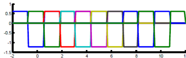
Fig (4), Second derivative of second degree B-spline basis function with uniform Knot vector X= \{-2,-1, 0, 1, 2, 3, 4, 5, 6, 7, 8, 9, 10, 11, 12\}
